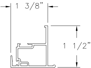
LOCK RAIL (4007) EXTRUDED RIGID PVC
